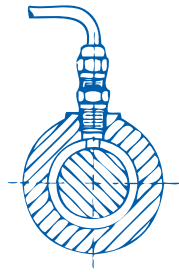
FIGURE 7.4 Tee Mounting
