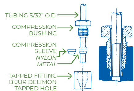
FIGURE 7.1 Compression Bushing
